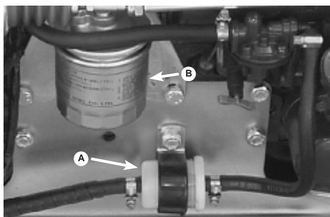
Figure 7.3 - Fuel Filter
