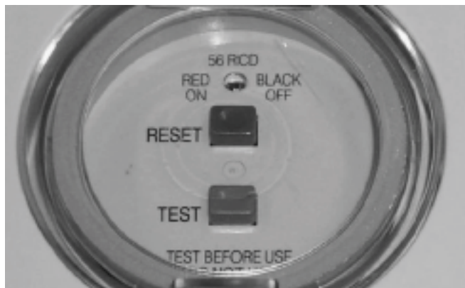
Figure 7.30 - RCD /ELCB
